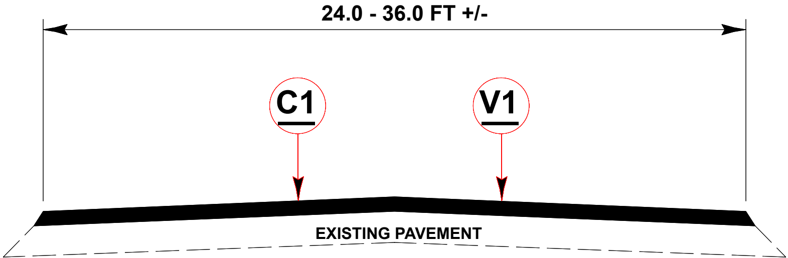
TYPICAL SECTION # 1 MAP(S) # 1- 3
