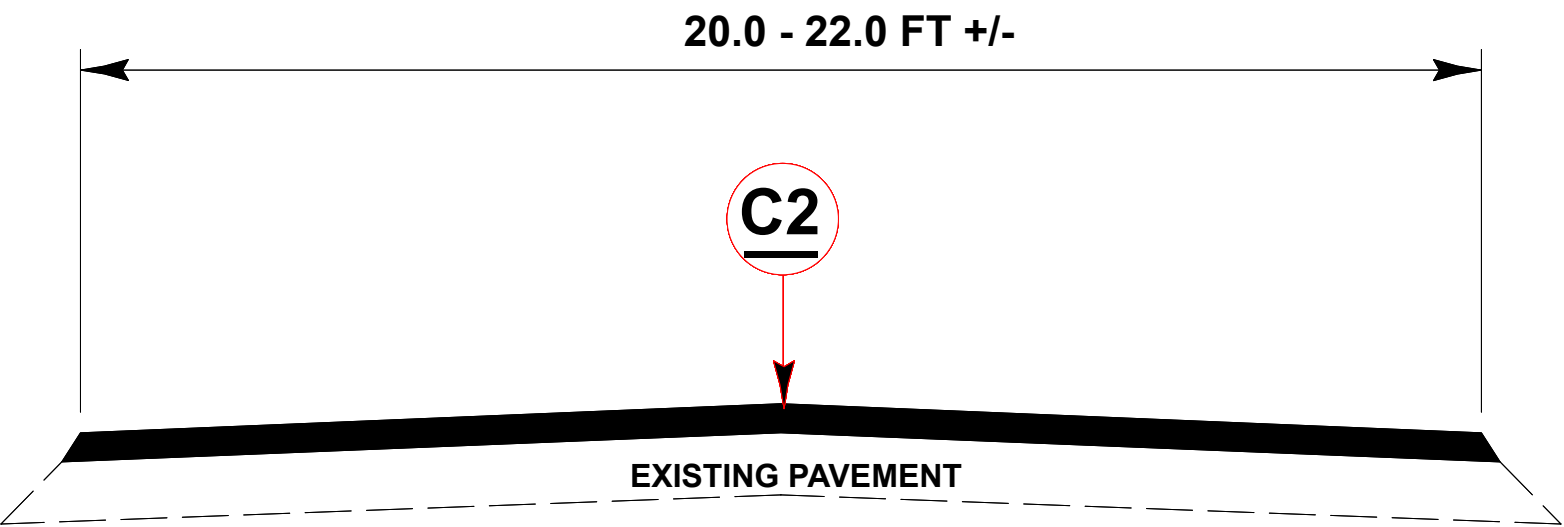
TYPICAL SECTION # 3 MAP(S) # 4 - 7
