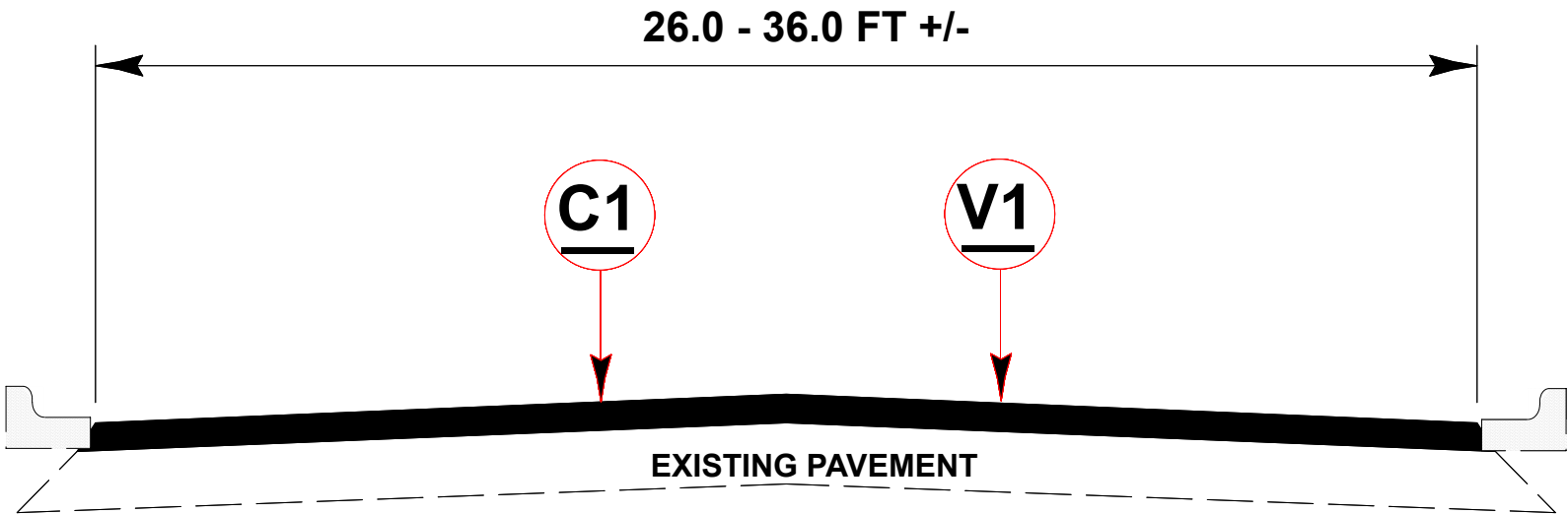
TYPICAL SECTION # 2 MAP(S) # 1 - 3
